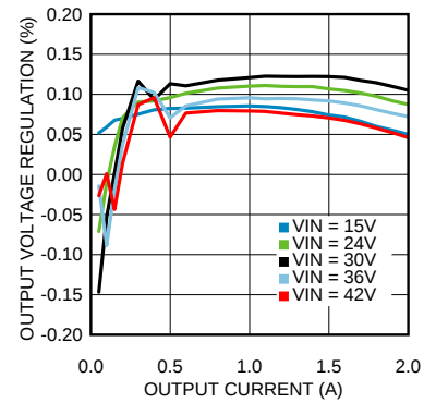
Figure 32. Line and Load Regulation T_A = 25^\circ\text{C}
