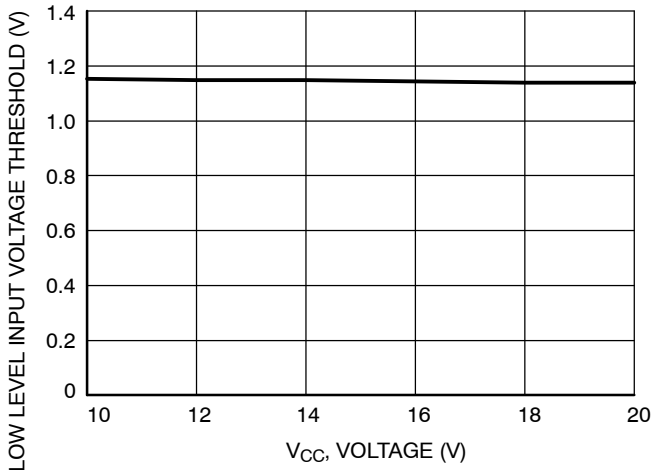
Figure 20. Low Level Input Voltage Threshold vs. Supply Voltage ( V_{CC} = V_{BOOT} )
