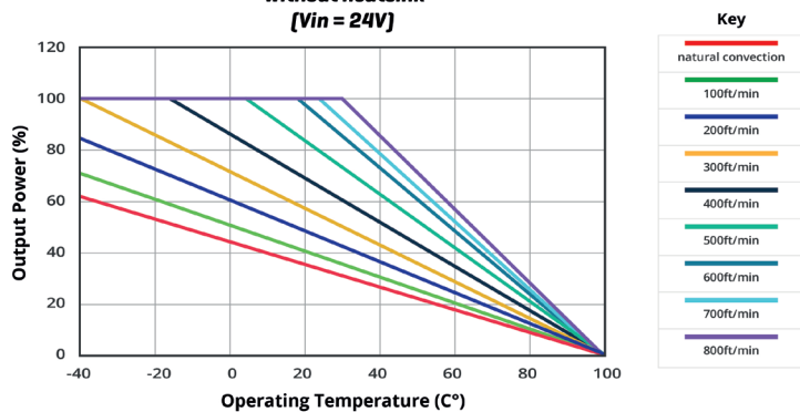
TEMPERATURE DERATING CURVE VHB350-D24-S12/S28 without heatsink ( V_{in} = 24V )
