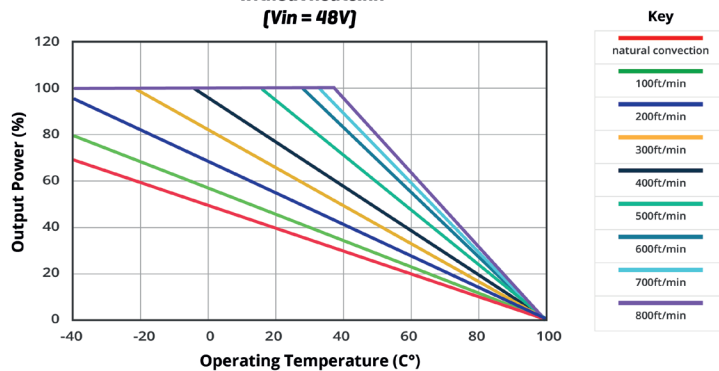
TEMPERATURE DERATING CURVE VHB350-D48-S12 without heatsink ( V_{in} = 48V )
