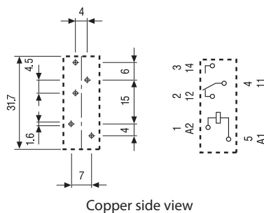
Copper side view
