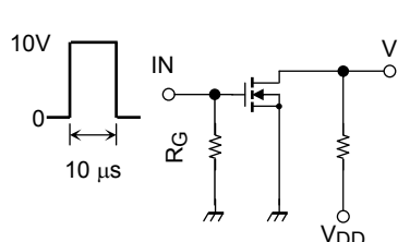
(a) Test Circuit
