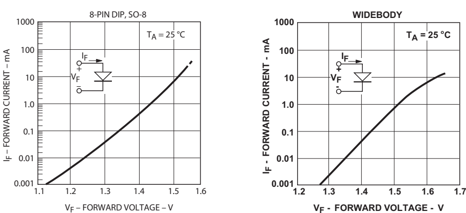
Figure 6: Typical Input Diode Forward Characteristic
