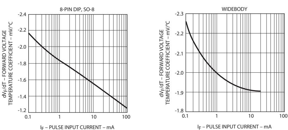
Figure 7: Typical Temperature Coefficient of Forward Voltage vs. Input Current
