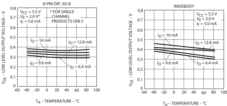
Figure 4: Typical Low Level Output Voltage vs. Temperature
