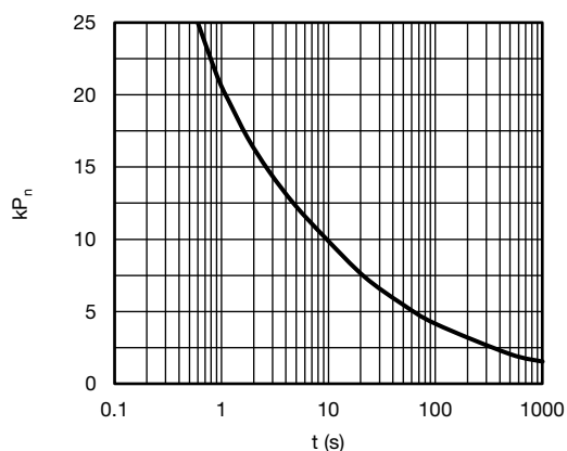
Intermittent Overloads Exceptional Operation Initial Temperature < 70^\circ\text{C} k \times P_n = f(t)
