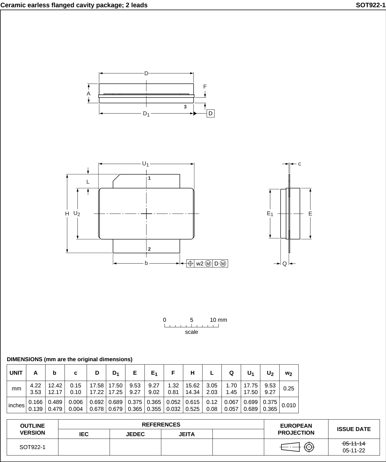
Fig 8. Package outline SOT922-1
