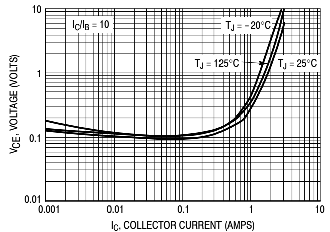
Figure 6. Collector-Emmitter Saturation Voltage
