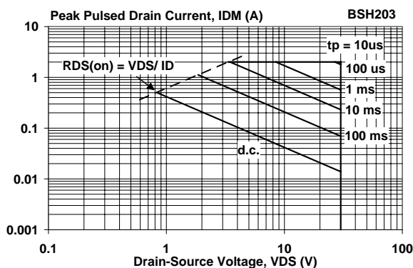
Fig. 3. Safe operating area. T_a = 25 \text{ } ^\circ\text{C} I_D \text{ \& } I_{DM} = f(V_{DS}) ; I_{DM} single pulse; parameter t_p
