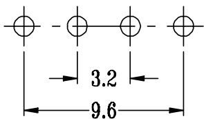
Recommended PCB Layout Top View
