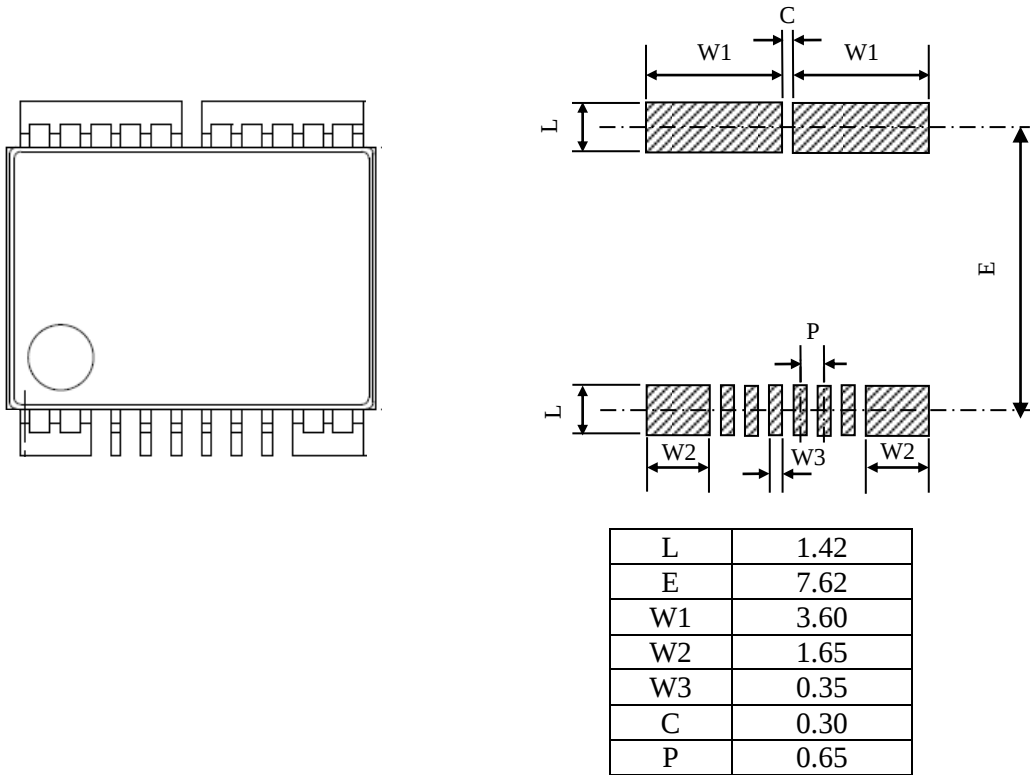
Figure 10. Pad dimensions of CQ-3202.
