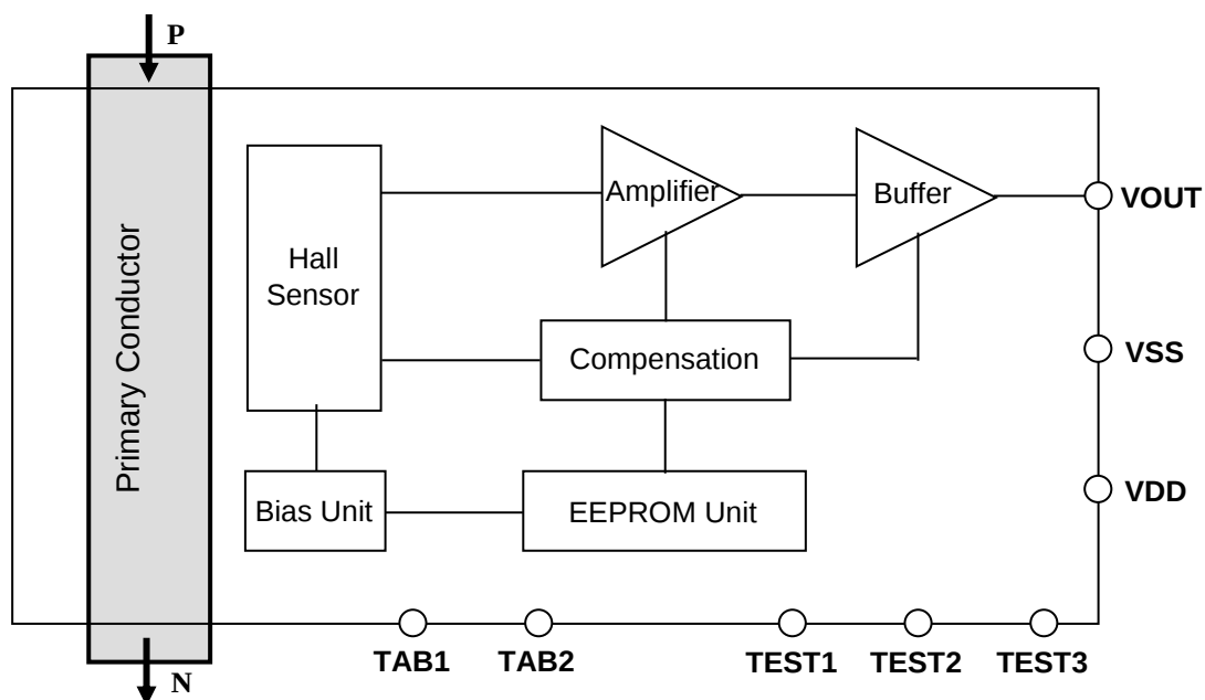
Figure 1. Functional block diagram of CQ-3202.
