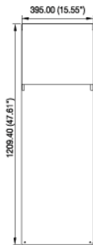
Front View
