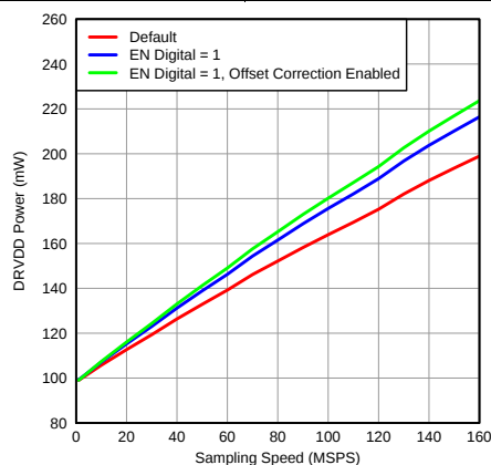
Figure 128. Digital Power in Various Modes (LVDS)
