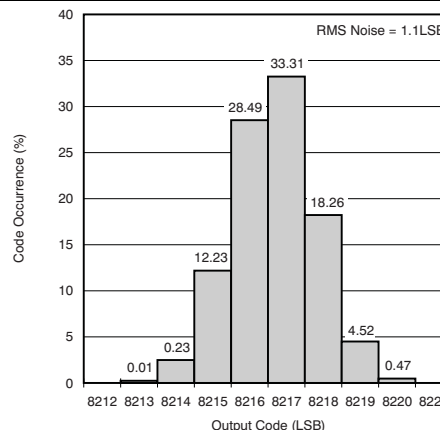
Figure 69. Output Noise Histogram (With Inputs Shorted to VCM)
