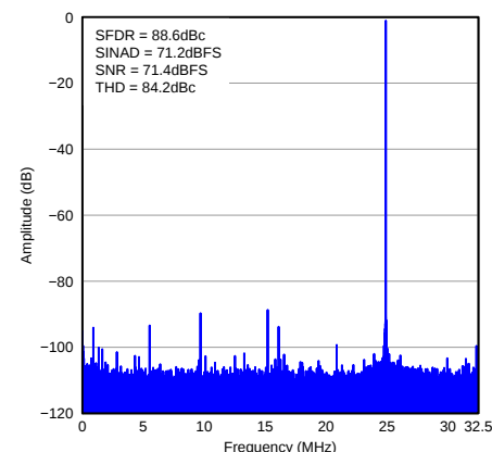
Figure 49. FFT for 170-MHz Input Signal
