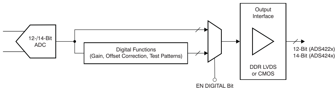
Figure 149. Digital Processing Block
