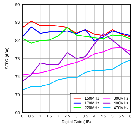
Figure 77. SFDR vs Gain and Input Frequency
