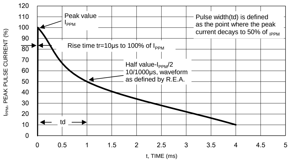
Fig.8 Pulse Waveform
