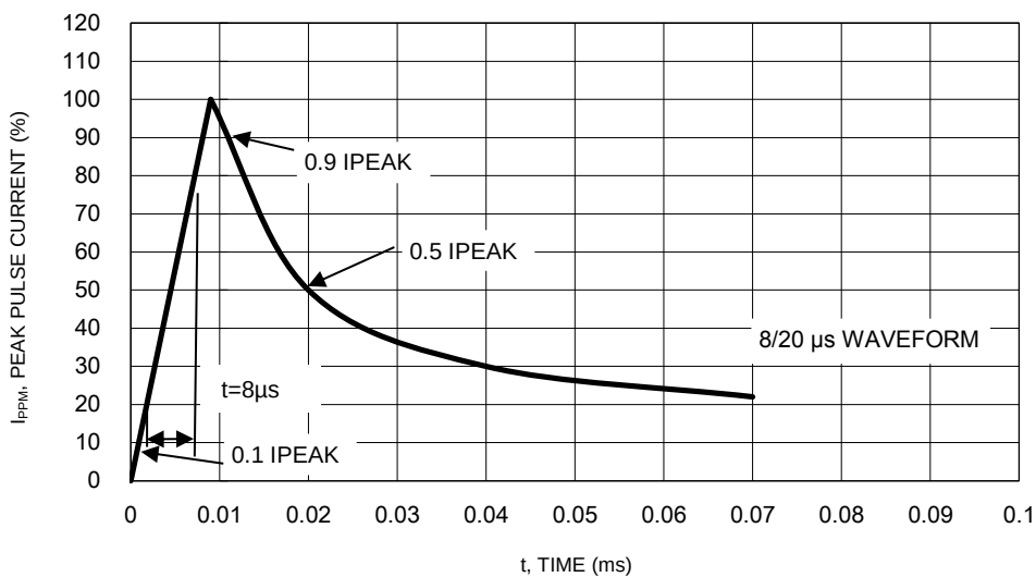
Fig.8 Pulse Waveform
