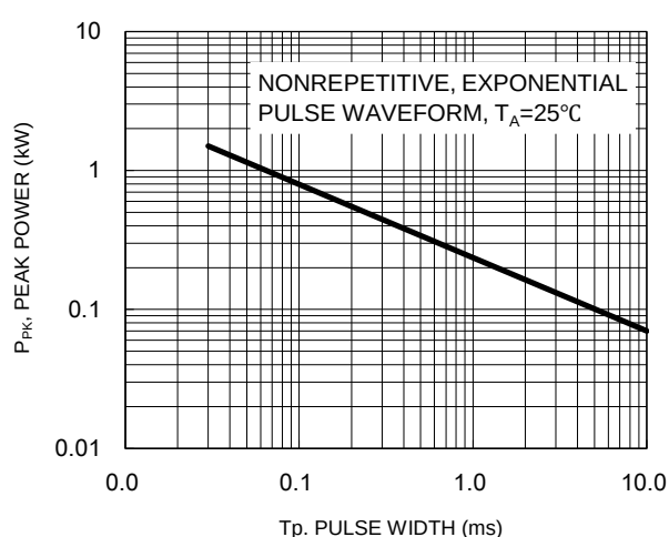
Fig.6 Typical Pulse Rating Curve
