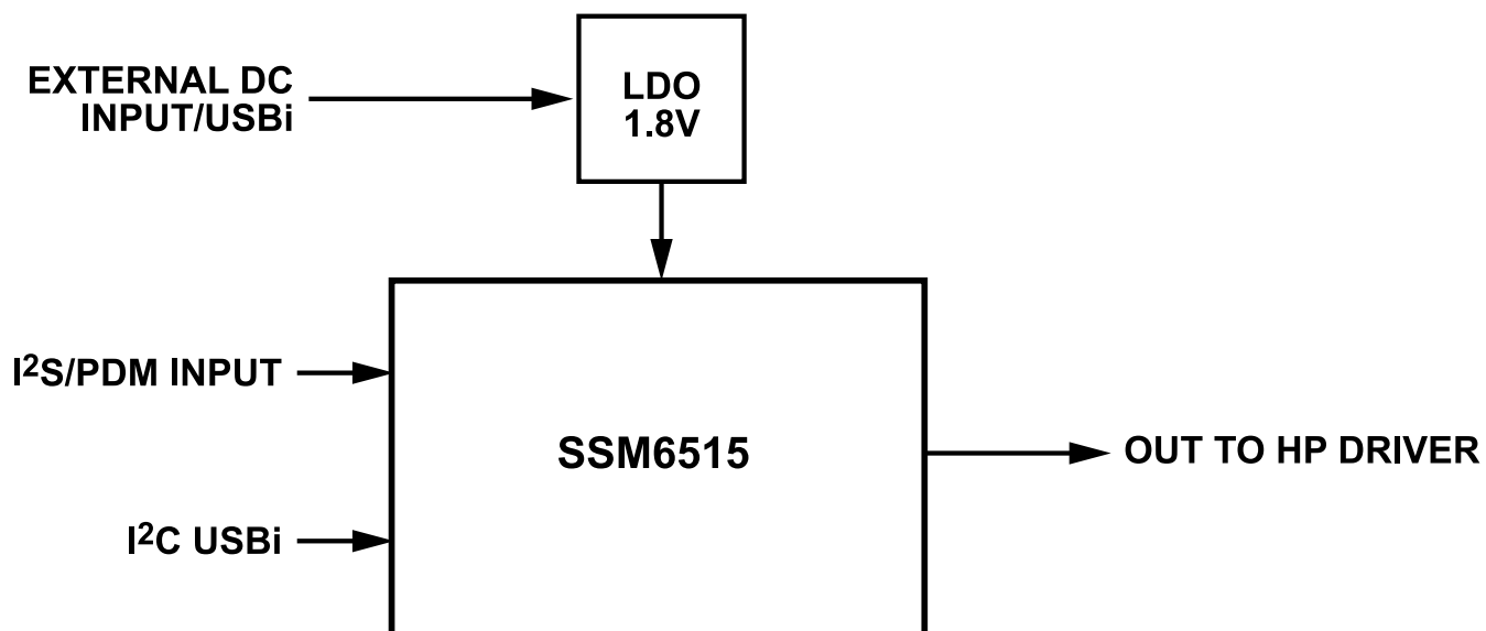
Figure 26. EVAL-SSM6515Z Schematic: Block Diagram (HP Is Headphone)
