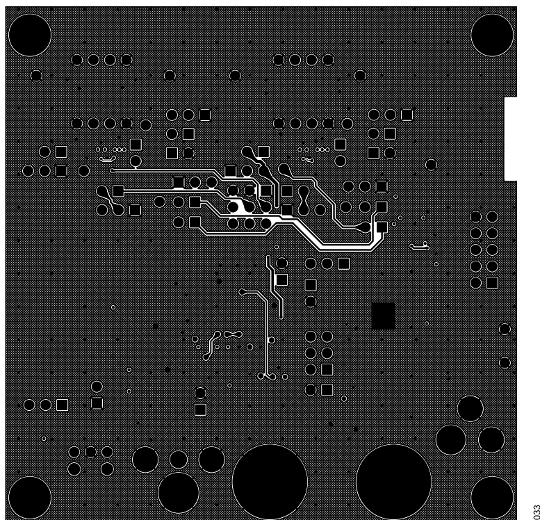
Figure 33. EVAL-SSM6515Z Layout: Bottom Copper
