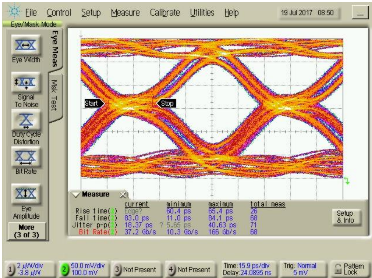
Figure 10: Eye diagram of GSSG configuration at 10.3125Gbps
