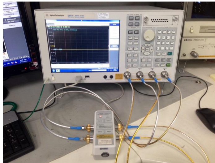
Figure 4: Network analyzer with eCal module
