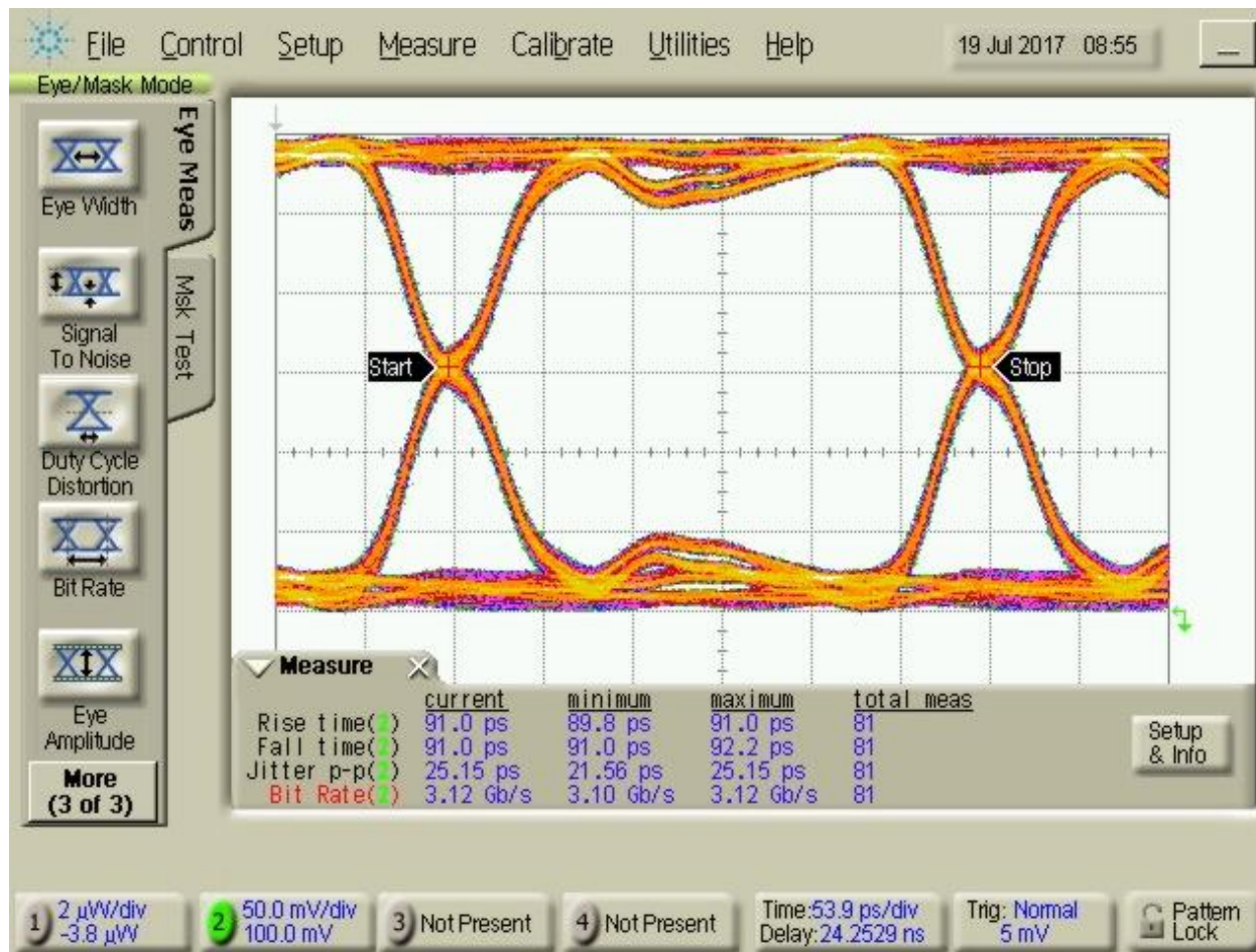
Figure 12: Eye diagram of DGSSG configuration at 3.125Gbps
