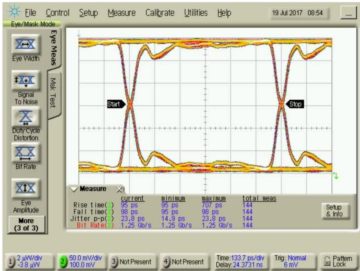
Figure 11: Eye diagram of DGSSG configuration at 1.25Gbps
