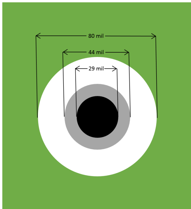
Figure D2. HD Stacker PCB Pad Geometry
