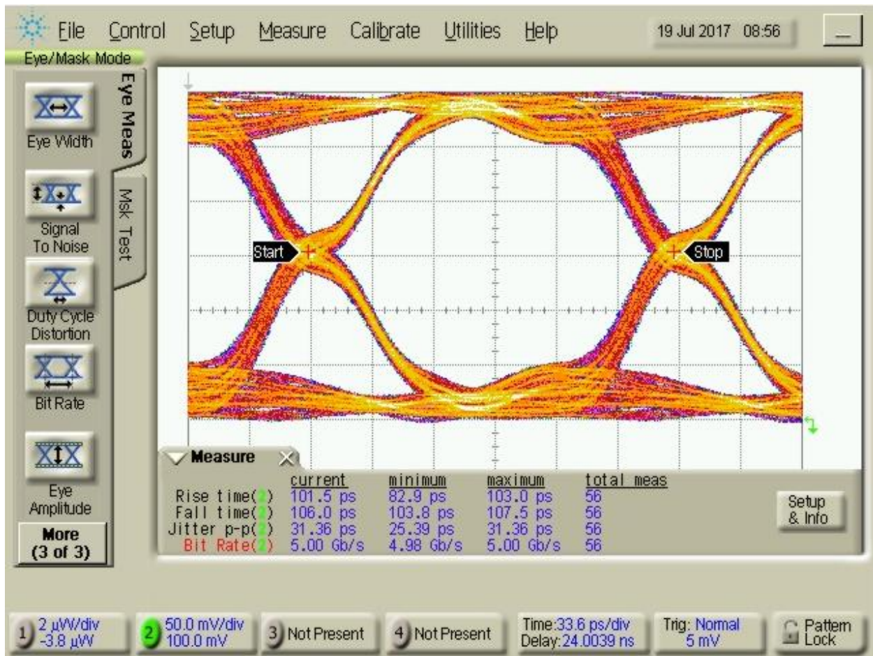
Figure 13: Eye diagram of DGSSG configuration at 5Gbps
