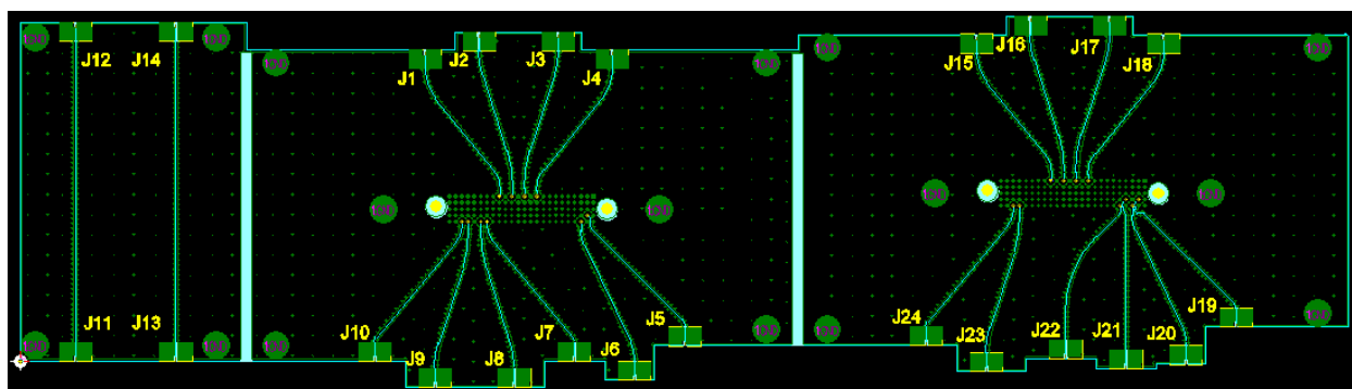
Figure 13. Test Fixture PCB layout
