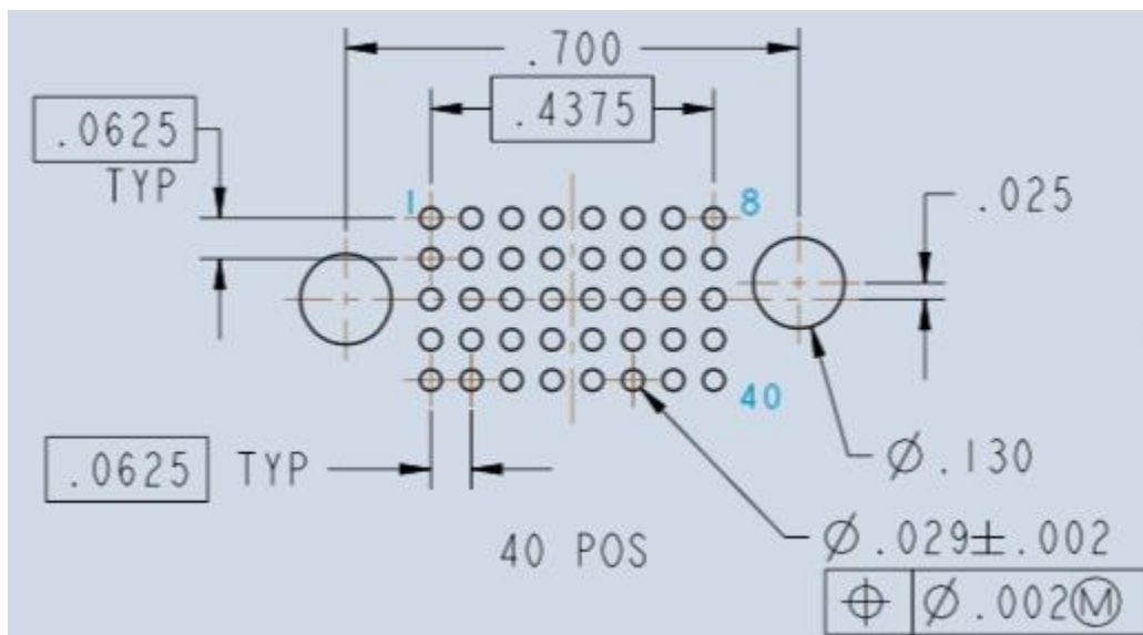
Figure D1. PCB Footprint for the 40 pin HD Stacker Connector.
