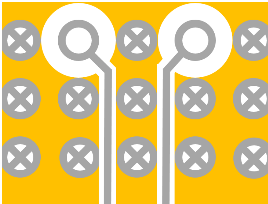
Figure D3. Inner Row Escape Routing
