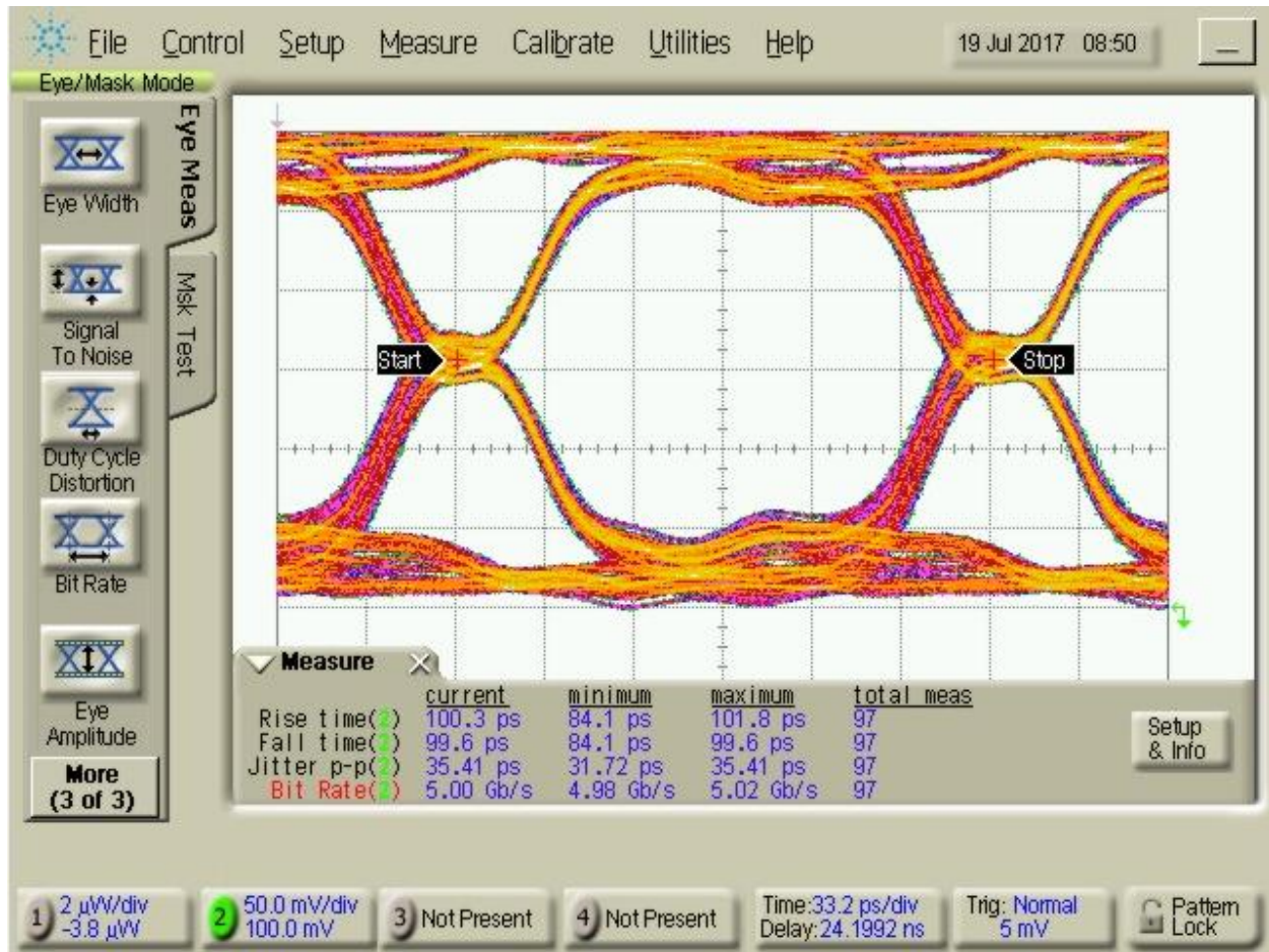
Figure 9: Eye diagram of GSSG configuration at 5Gbps
