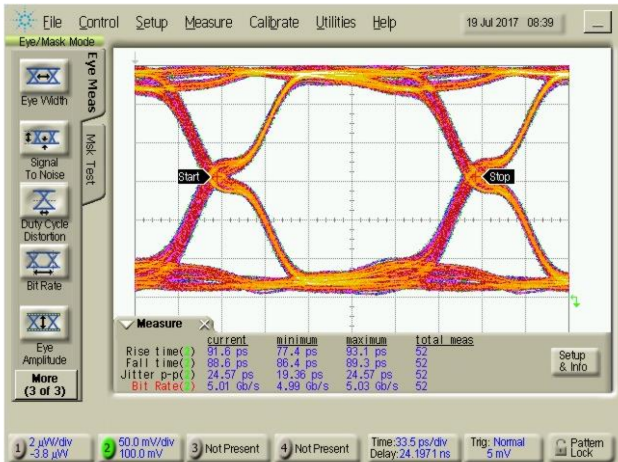
Figure 5: Eye diagram of GSGSG configuration at 5Gbps
