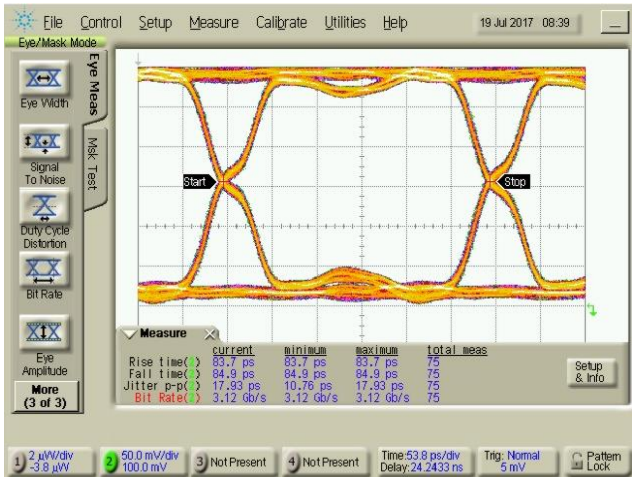
Figure 4: Eye diagram of GSGSG configuration at 3.125Gbps
