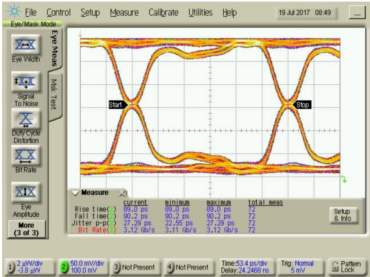
Figure 8: Eye diagram of GSSG configuration at 3.125Gbps
