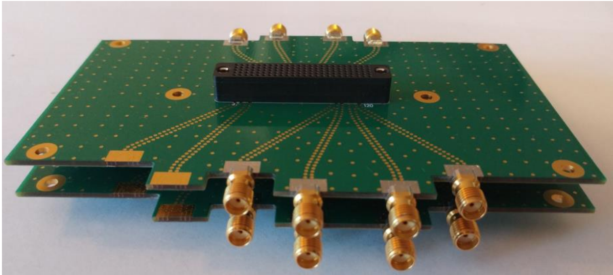
Figure 2. Stacked Test PCBs
