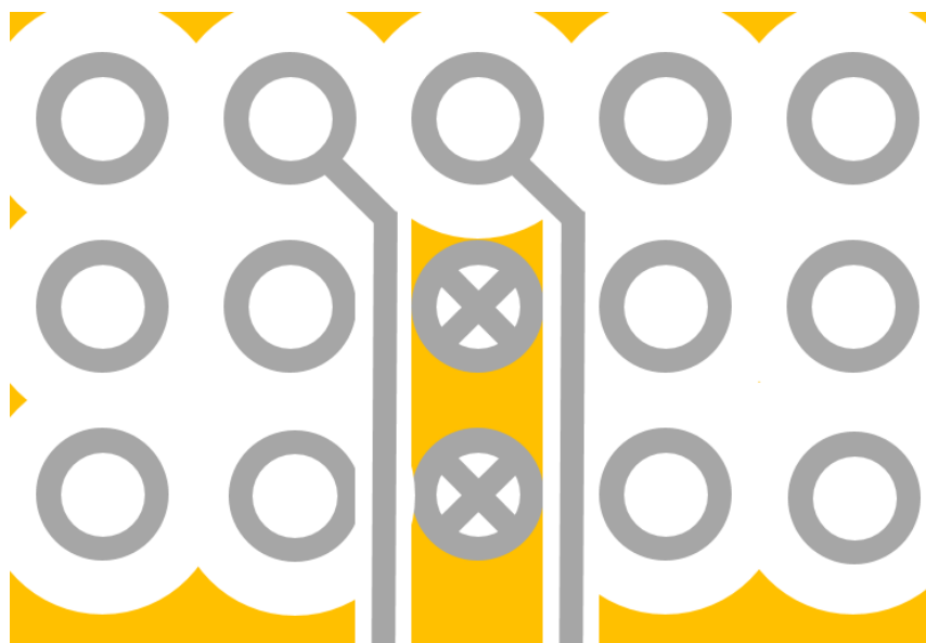
Figure D4. Alternate Inner Row Escape Routing
