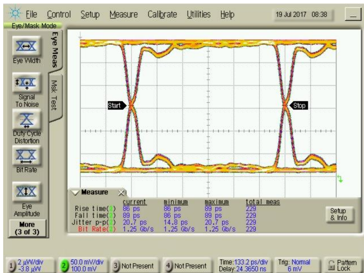
Figure 3: Eye diagram of GSGSG configuration at 1.25Gbps
