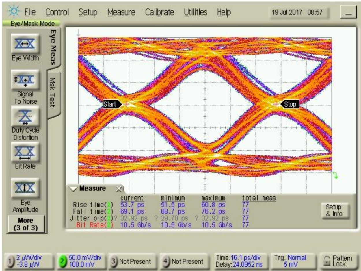
Figure 14: Eye diagram of DGSSG configuration at 10.3125Gbps
