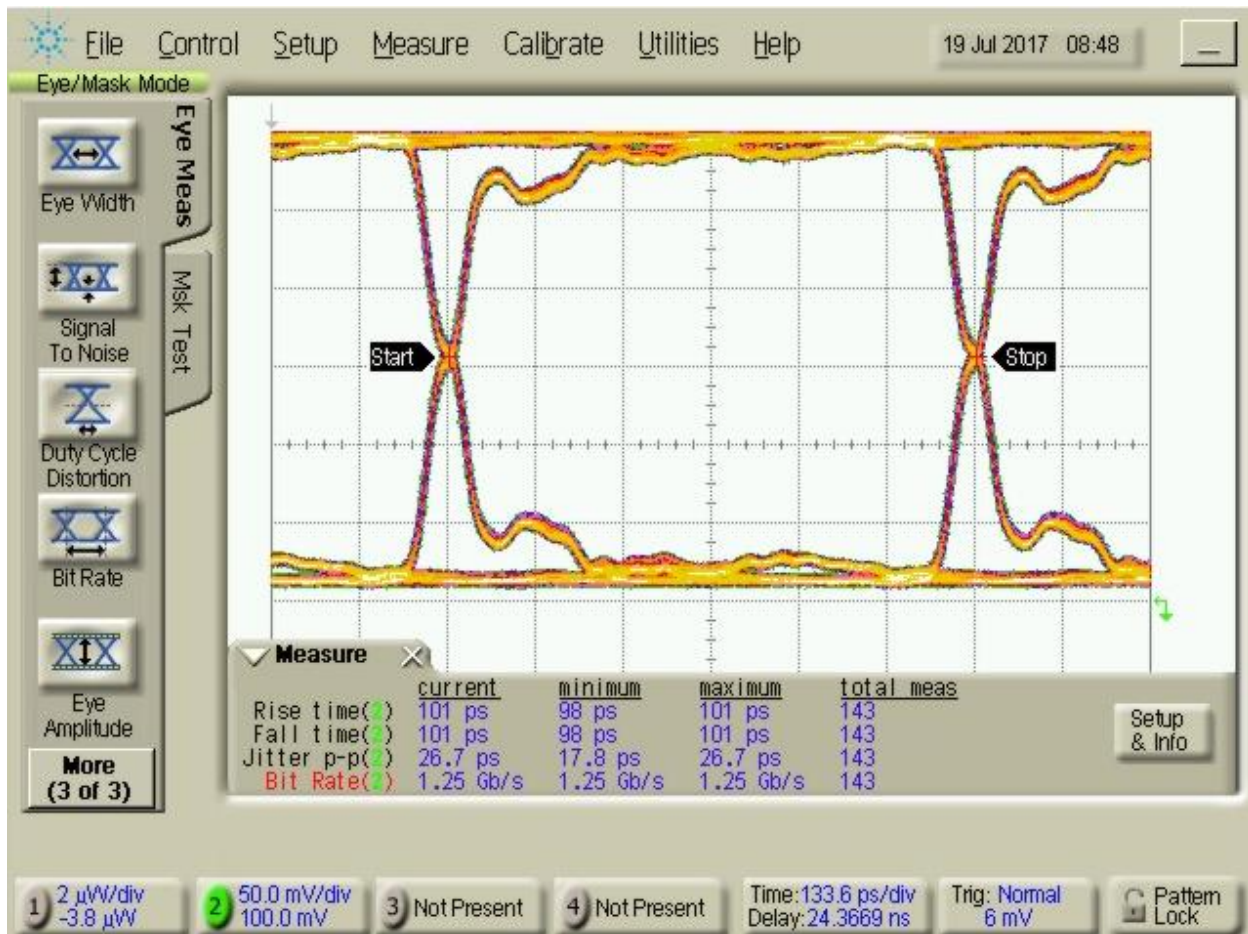
Figure 7: Eye diagram of GSSG configuration at 1.25Gbps
