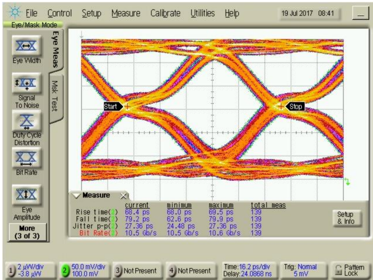
Figure 6: Eye diagram of GSGSG configuration at 10.3125Gbps
