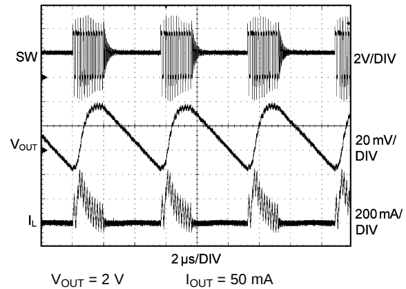
Figure 25. Output Voltage Ripple in ECO Mode
