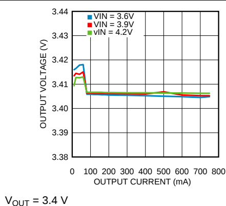
Figure 6. Output Voltage vs Output Current
