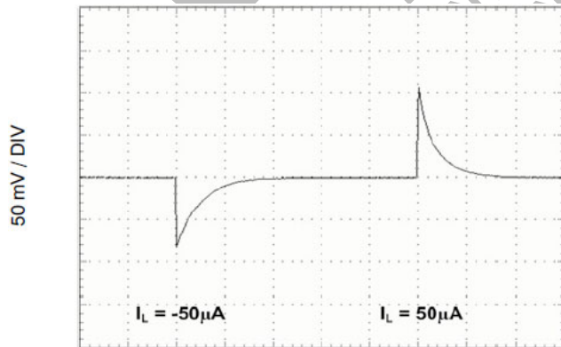
Figure 12. Load Transient ( I_L = 50 \mu\text{A} )
