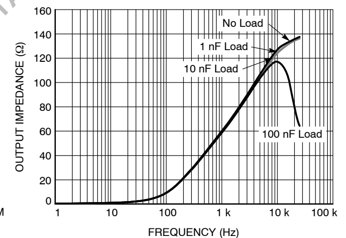
Figure 7. Output Impedance vs. Frequency
