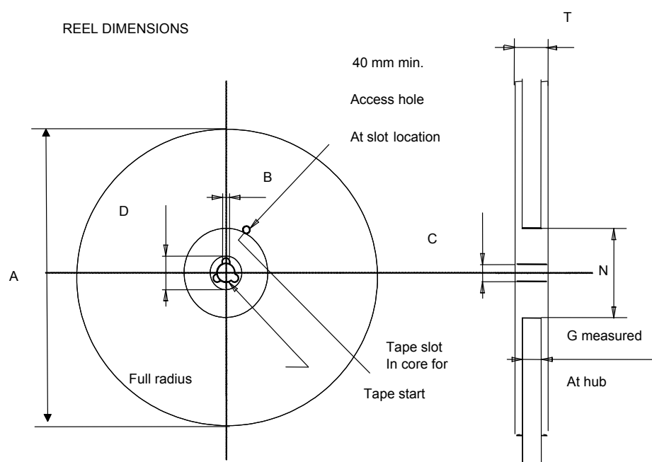
Figure 34. Reel outline
