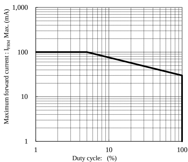
Max. forward current vs. Duty cycle
