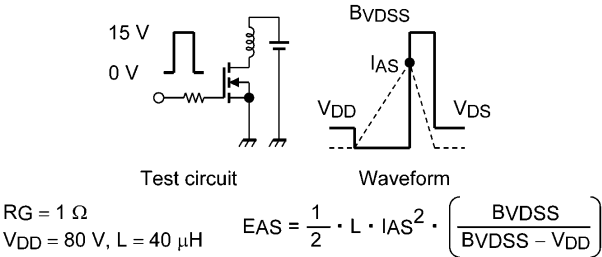
Fig. 8.17 Test Circuit/Waveform
