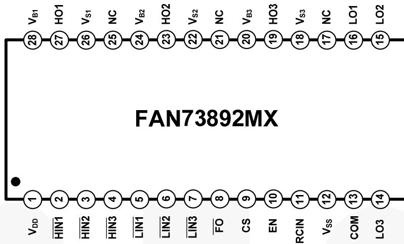
Figure 3. Pin Assignments
