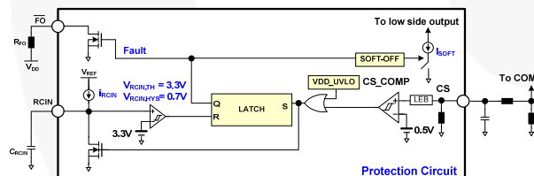
Figure 41. Over-Current Protection
