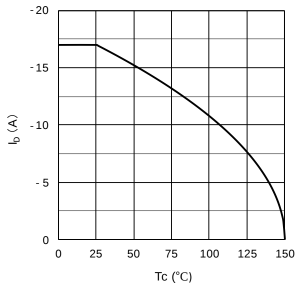
I_D - T_c characteristics
