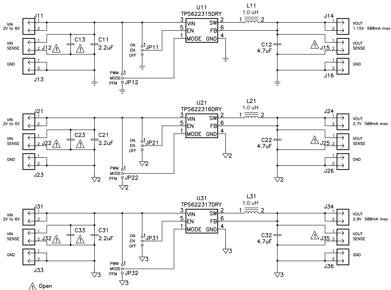
Figure 4. TPS622315/316/317EVM-574 Schematic
