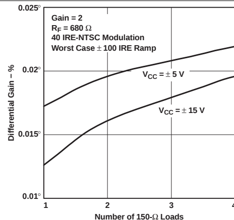
Figure 40. Differential Gain vs Number of 150-Ω Loads
