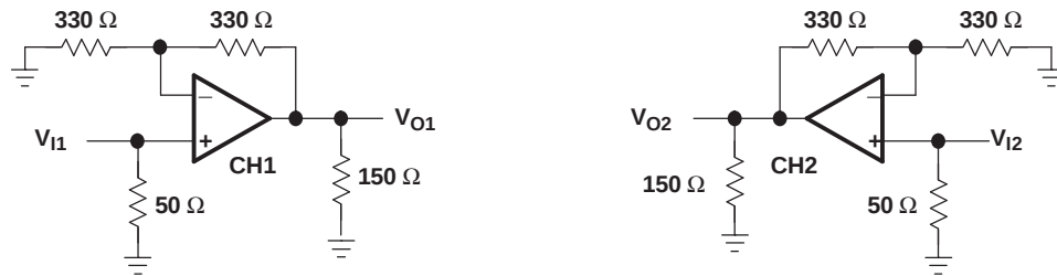
Figure 46. THS4032 Crosstalk Test Circuit
