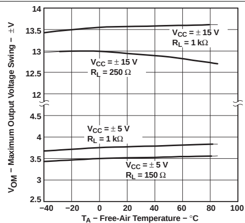
Figure 6. Maximum Output Voltage Swing vs Free-Air Temperature
