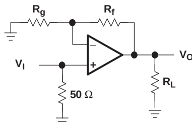
Figure 47. Step Response Test Circuit
