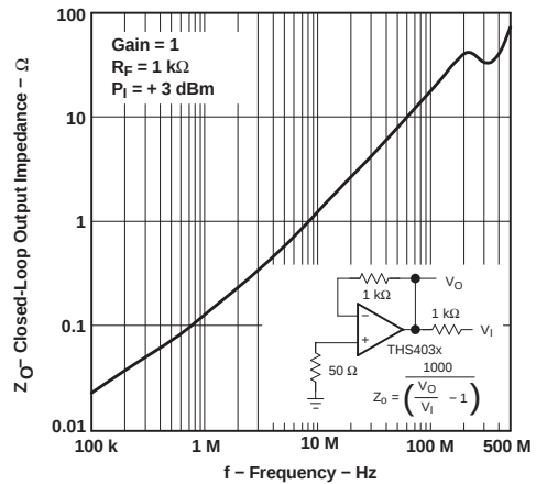
Figure 10. Closed-Loop Output Impedance vs Frequency
