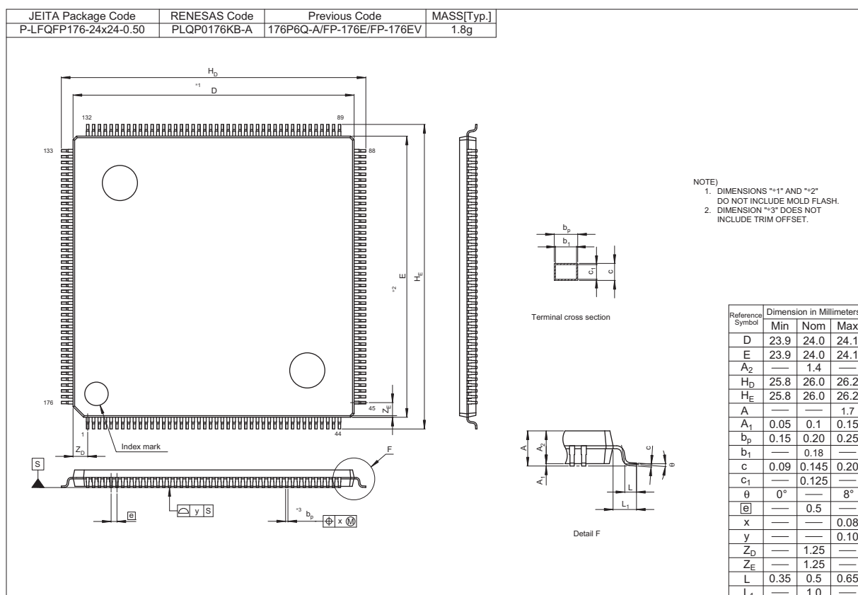
Figure 1.2 176-pin LQFP
