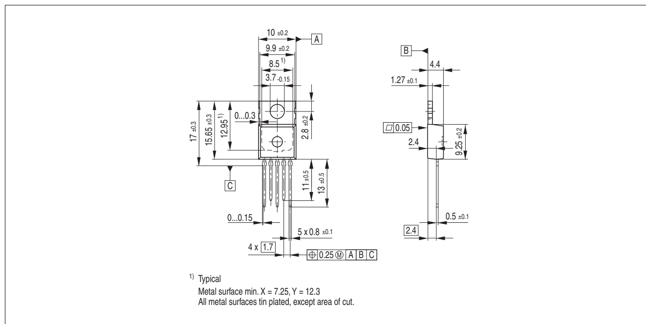
Figure 6 PG-TO220-5 1)
