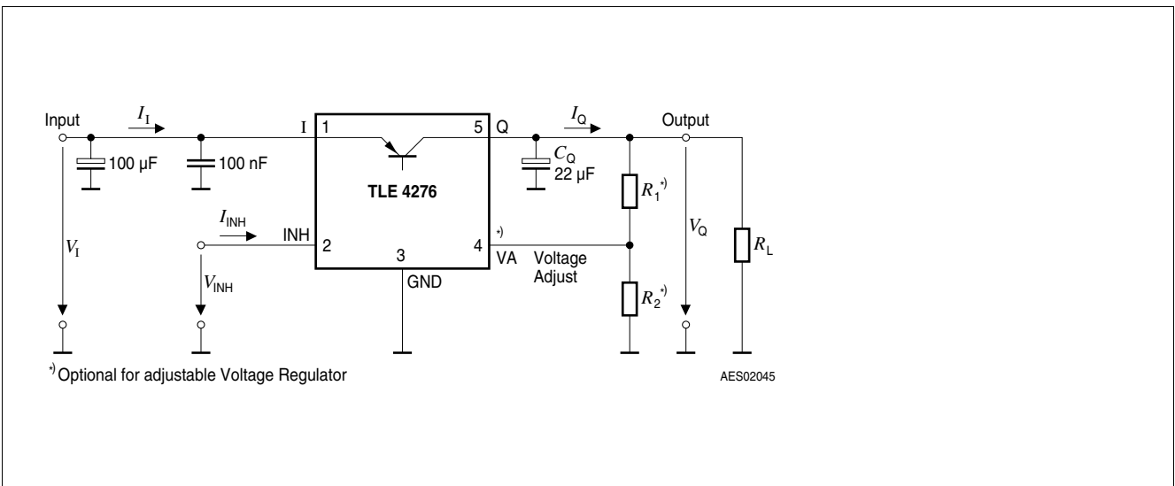
Figure 3 Measuring Circuit
