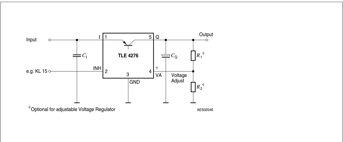
Figure 4 Application Circuit
