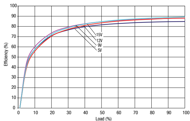
MEE3S12xxSC Input Voltage
