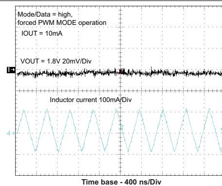
Figure 31. Output Voltage Ripple In Forced PWM Mode
