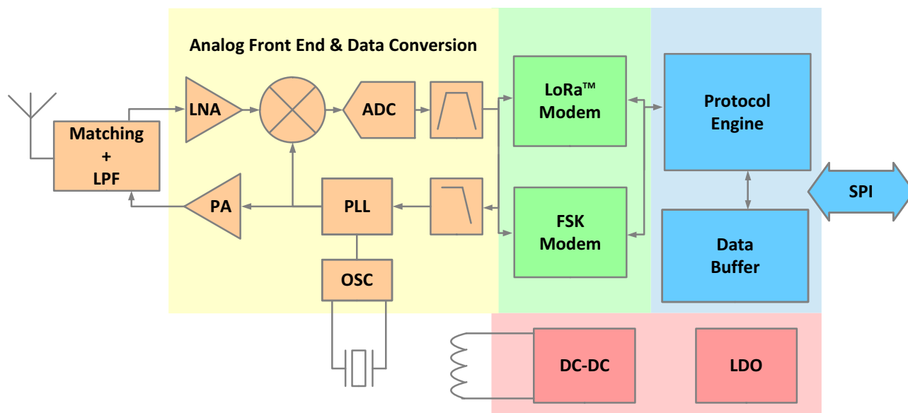
Figure A: LLCC68 Block Diagram
