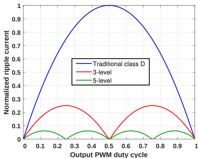
Figure 11.3: Ripple current comparison
