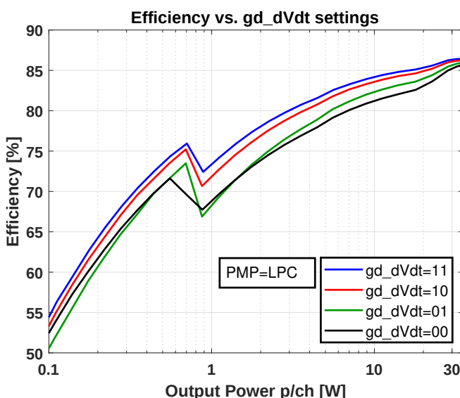
Figure 11.22: Efficiency for different gd_dVdt settings
