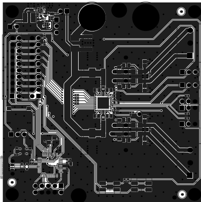
Figure 12.4: Top Layer
