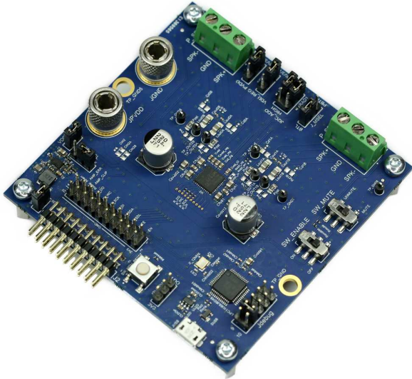
Figure 12.2: Evaluation board top side
