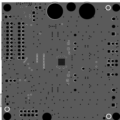
Figure 12.6: Mid Layer 2
