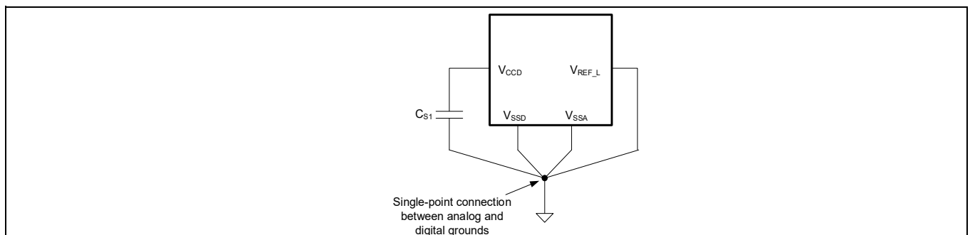
Figure 12 Smoothing capacitor
