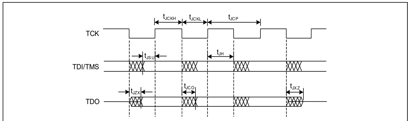
Figure 31 JTAG specifications
