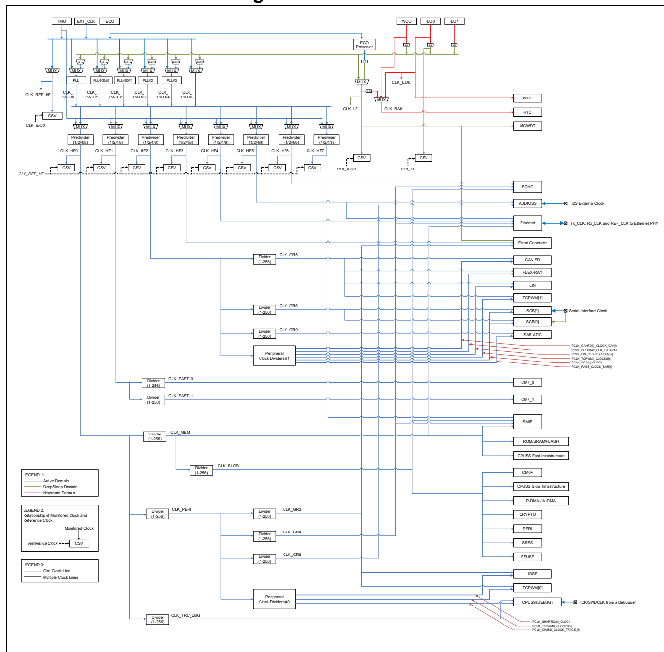
Figure 4 CYT4BF clock diagram
