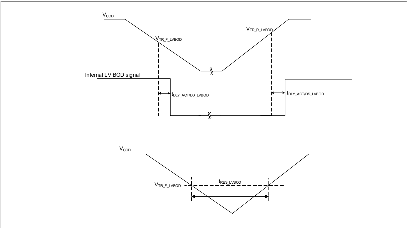
Figure 27 Low-voltage BOD specifications
