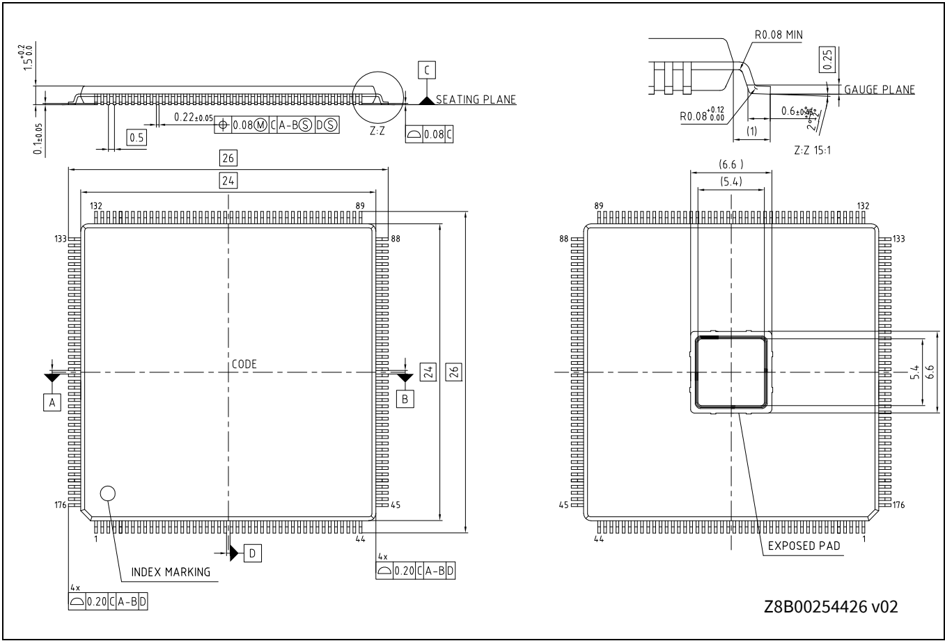
Figure 58 Package outline - 176-TEQFP
