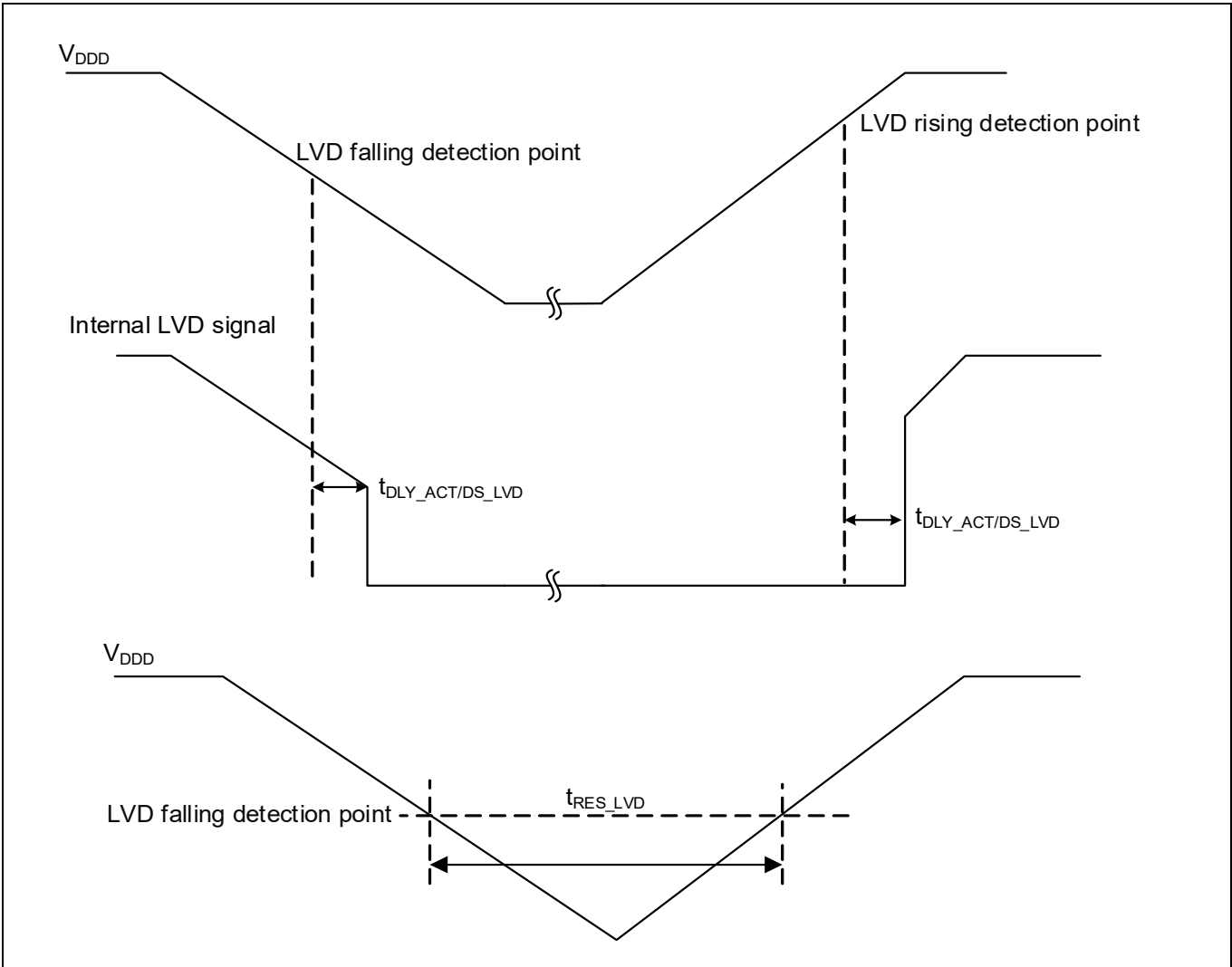
Figure 30 LVD specifications
