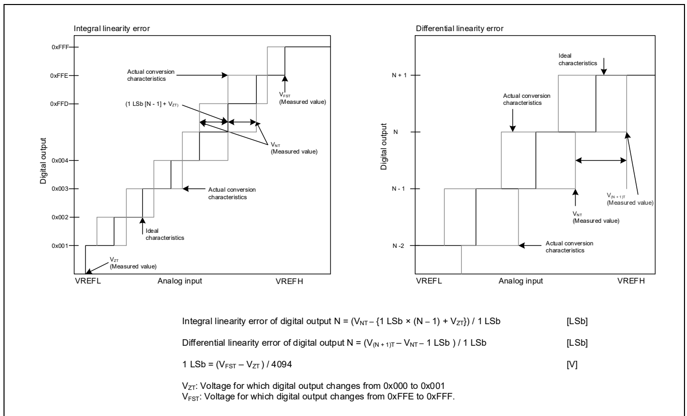
Figure 15 Integral and differential linearity errors
