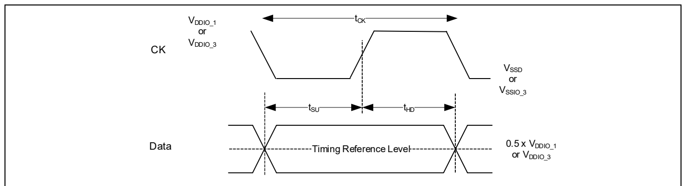
Figure 50 SDR write timing reference level
