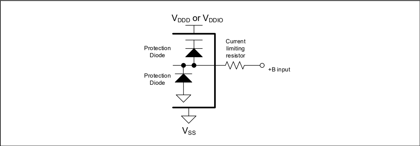
Figure 11 Example of a recommended circuit [45]
