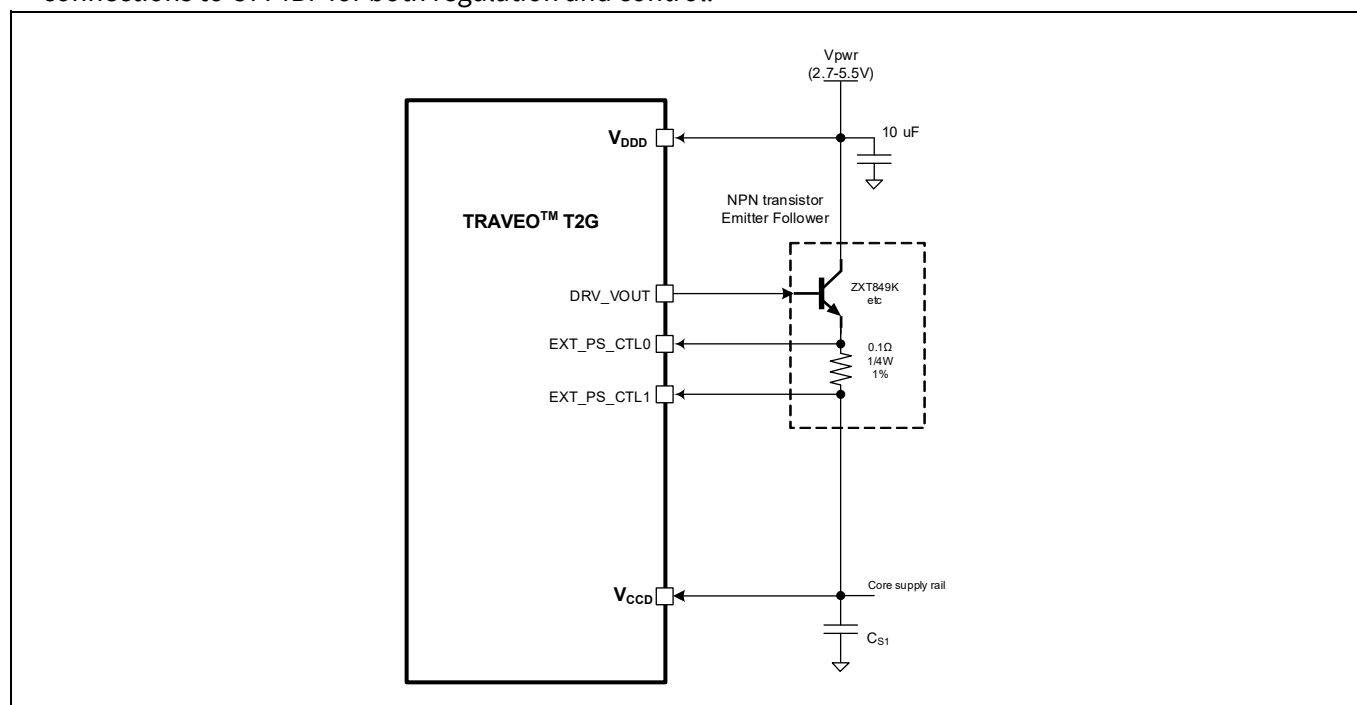
Figure 1 Sample core external regulator with NPN transistor
