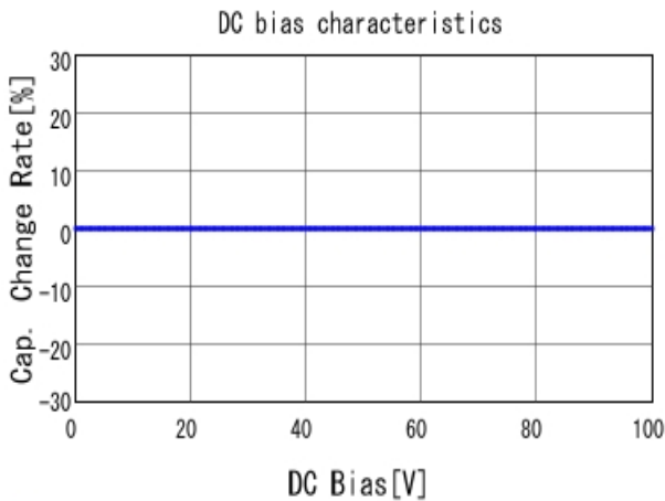
■ GRM1885C2A471JA01 C-DC bias capchange, 25.0degC, AC1V
