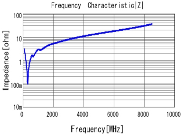
■ GRM1885C2A471JA01 |Z| DC0V, 25degC
