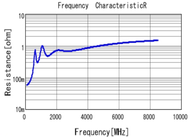
■ GRM1885C2A471JA01 R DC0V, 25degC
