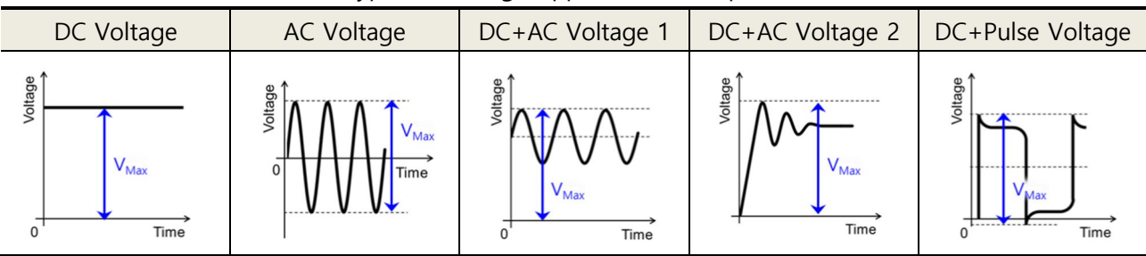
[Types of Voltage Applied to the Capacitor]
