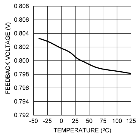
Figure 12. Feedback Pin Voltage vs Temperature
