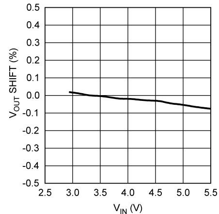
Figure 10. Line Regulation
