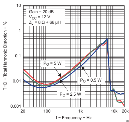
Figure 1. Total Harmonic Distortion vs Frequency (BTL)
