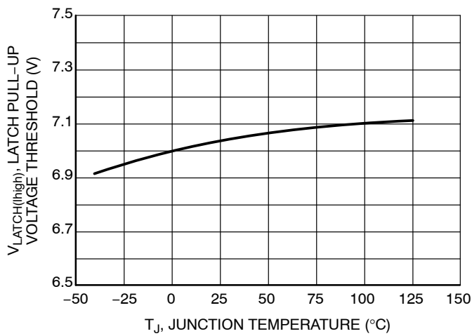
Figure 46. Latch Pull-Up Voltage Threshold vs. Junction Temperature
