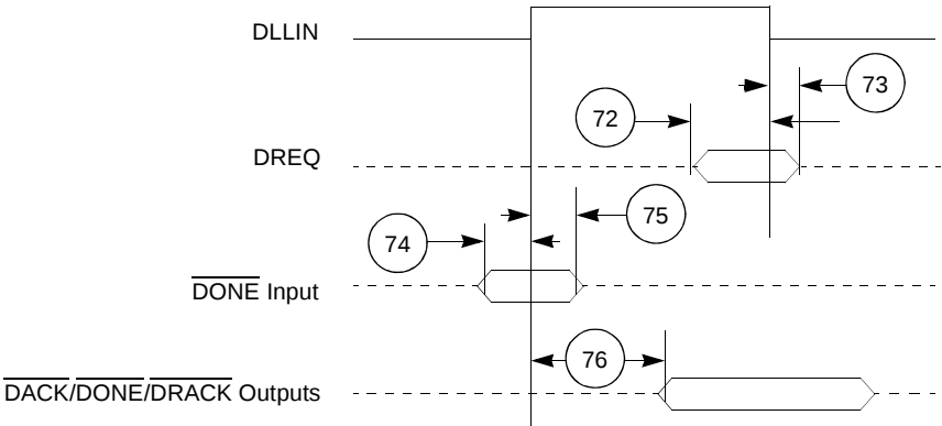
Figure 2-11. DMA Signals
