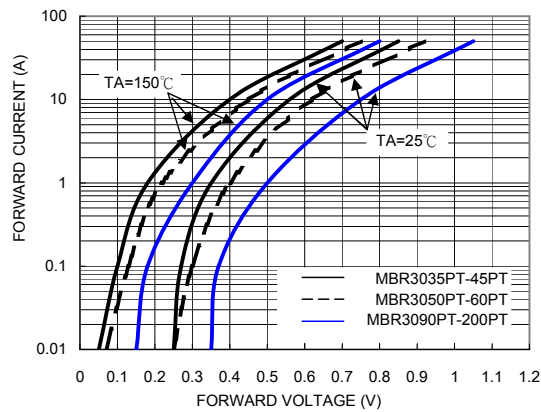
FIG. 3 TYPICAL FORWARD CHARACTERISRICS
