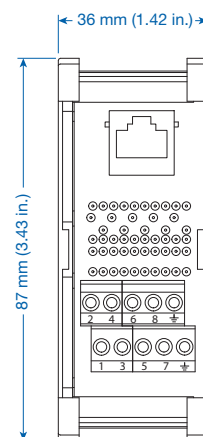
With Vertical - Top Entry RJ45 Connector
