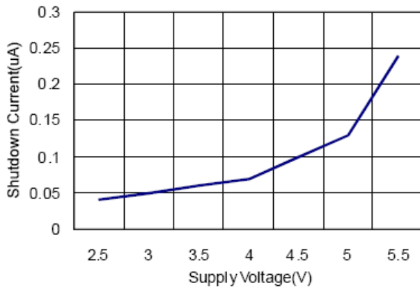
27. Shutdown Current
