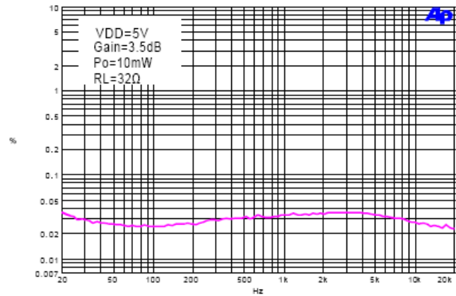
14. THD+N vs. Frequency
