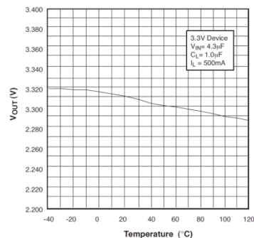
Fig. 14 Output Voltage vs Temperature
