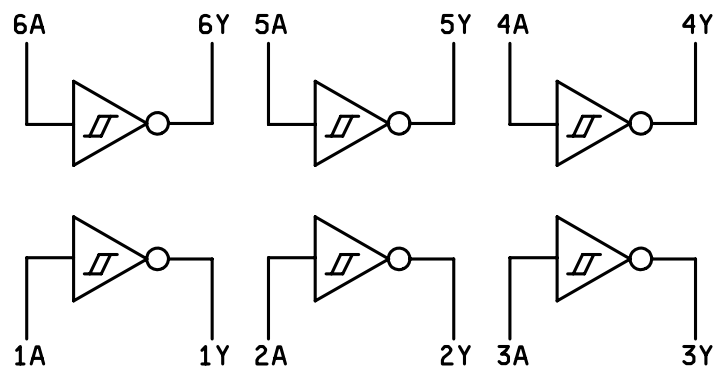
FIGURE 3. Logic diagram.
