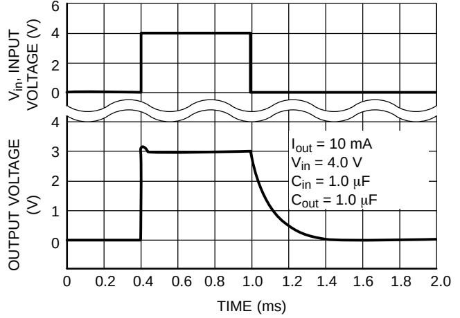
Figure 11. Turn-on Response
