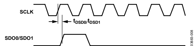
Figure 8. SCLK, SDO0/SDO1 Switching Characteristics
