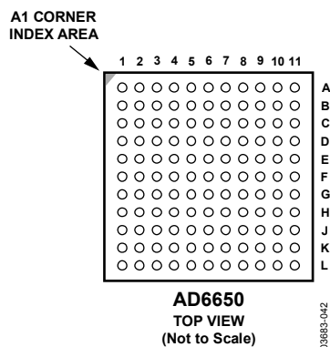
Figure 14. Pin Configuration
