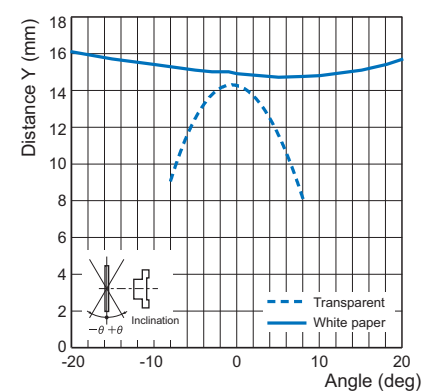
B5W-LB1
