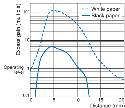
B5W-LB1
