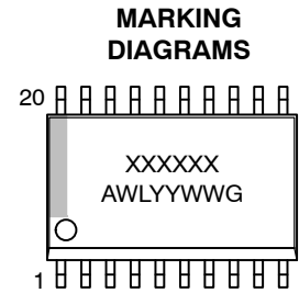
SOIC-20W DW SUFFIX CASE 751D
