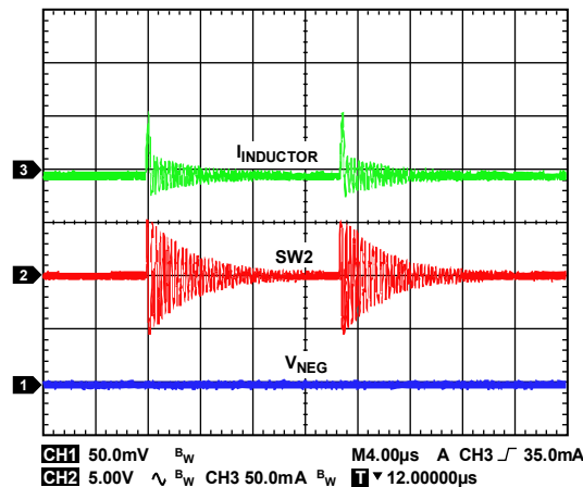
Figure 36. Inverting Regulator Skip Mode Operation Showing I_{INDUCTOR} , Switch Node Voltage, and Output Ripple, V_{IN} = +5\text{ V} , V_{NEG} = -5\text{ V} , I_{LOAD2} = 0\text{ mA} , f_{SW} = 2.4\text{ MHz} , T_A = 25^\circ\text{C}
