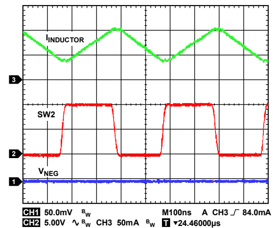
Figure 38. Inverting Regulator Continuous Conduction Mode Operation Showing I_{INDUCTOR} , Switch Node Voltage, and Output Ripple, V_{IN} = +5\text{ V} , V_{NEG} = -5\text{ V} , I_{LOAD2} = 35\text{ mA} , f_{SW} = 2.4\text{ MHz} , T_A = 25^\circ\text{C}
