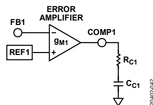
Figure 44. Compensation Components
