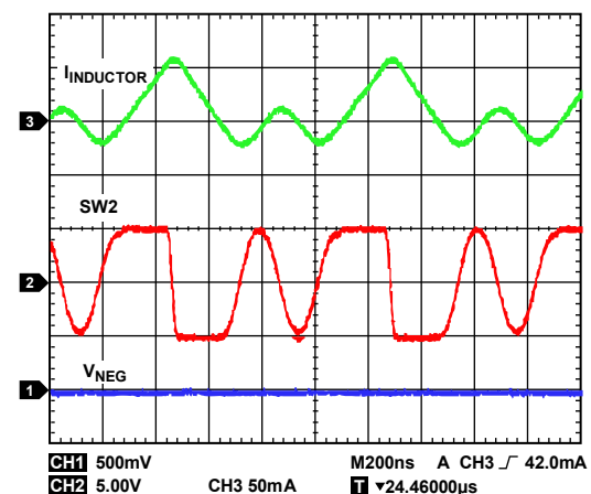
Figure 37. Inverting Regulator Discontinuous Conduction Mode Operation Showing I_{INDUCTOR} , Switch Node Voltage, and Output Ripple, V_{IN} = +5\text{ V} , V_{NEG} = -5\text{ V} , I_{LOAD2} = 6\text{ mA} , f_{SW} = 2.4\text{ MHz} , T_A = 25^\circ\text{C}
