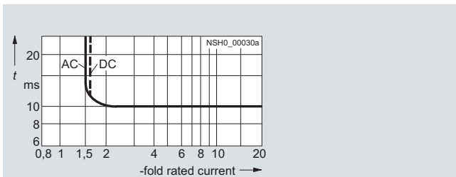
Tripping characteristics of short-circuit releases
